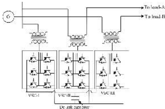
Fig. 1. Basic connection of GUPFC
