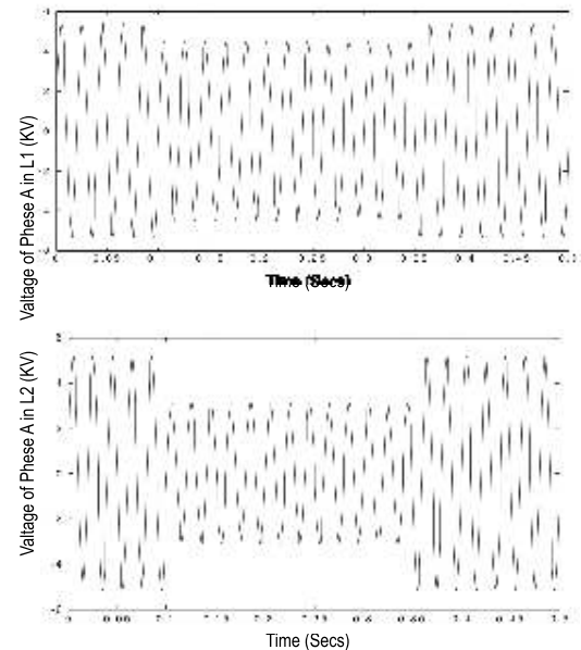
Fig.10. a. Uncompensated load voltage of lines L 2 b. Uncompensated load voltage of lines L 1 and L 2
