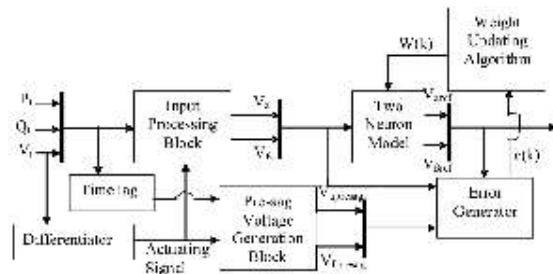
Fig. 6. Basic block diagram of proposed controller
