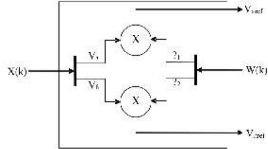
Fig. 9. Two-Neuron model
