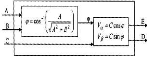
Fig. 7. Input processing /Pre-sag voltage generation block
