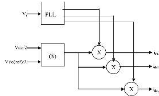
Fig. 4. Three-phase self charging circuit
