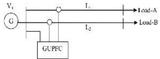
Fig. 2. Basic connection of GUPFC
