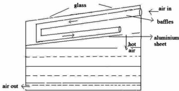
Fig. 1 Two pass Air heater with drying chamber
